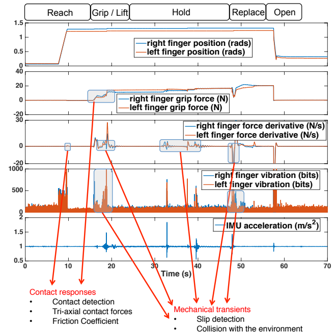
Fig. 11: An example run of the grip controller that includes all of the grasping phases.
