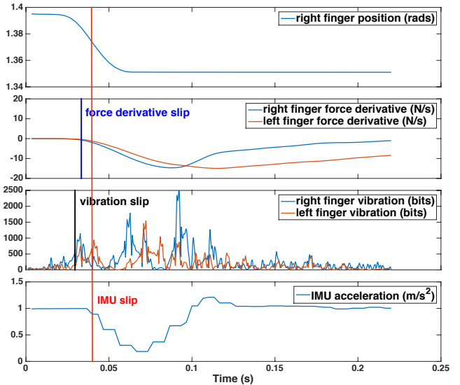
Fig. 8: An example run of the slip detection experiment. Using the BioTac sensor we are able to detect the slip event before the IMU accelerometer attached to the object measures any acceleration due to slip.
